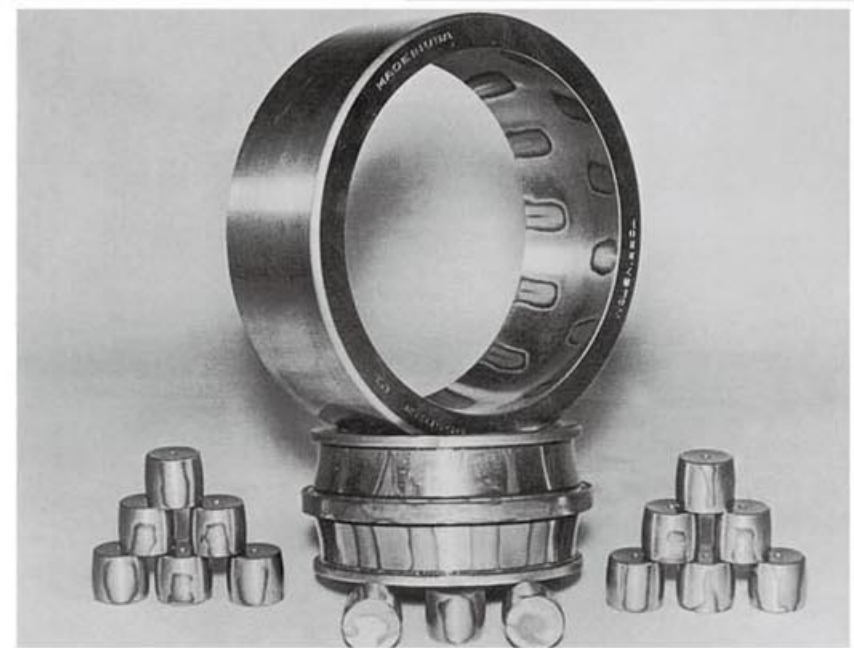
Figure 1 STAINING IN STORAGE
