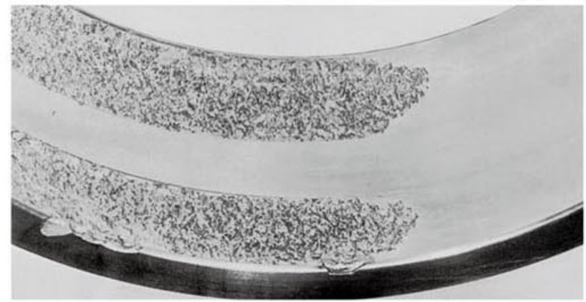
Figure 34 FATIGUE
