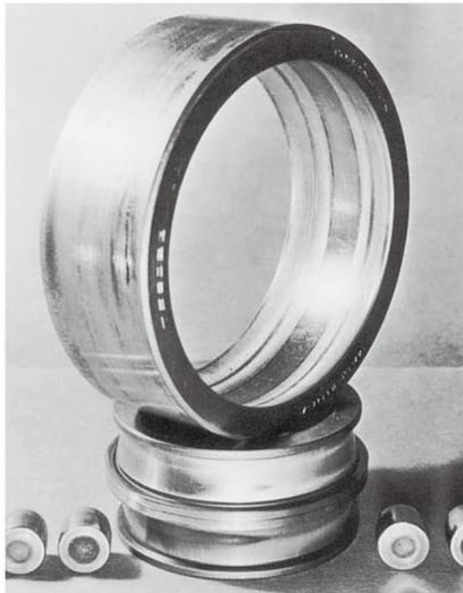
Figure 29 ABRASIVE WEAR - RINGS AND ROLLERS
