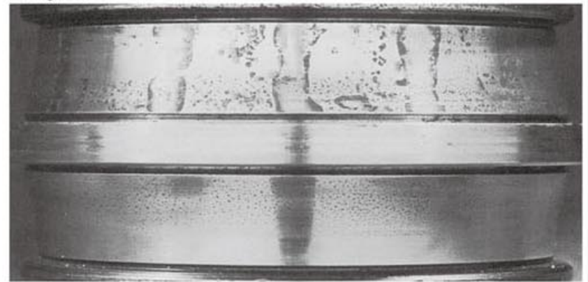
Figure 5 CORROSION AND FAILURE
