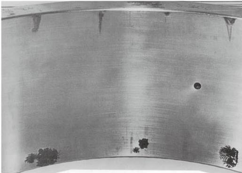
Figure 6 CORROSION IN STORAGE
