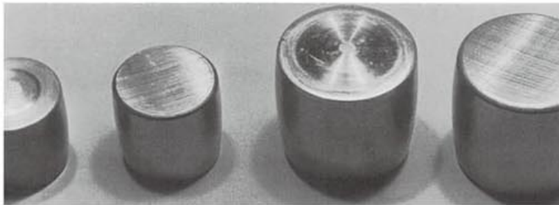
Figure 32 ABRASIVE WEAR-ROLLER END
