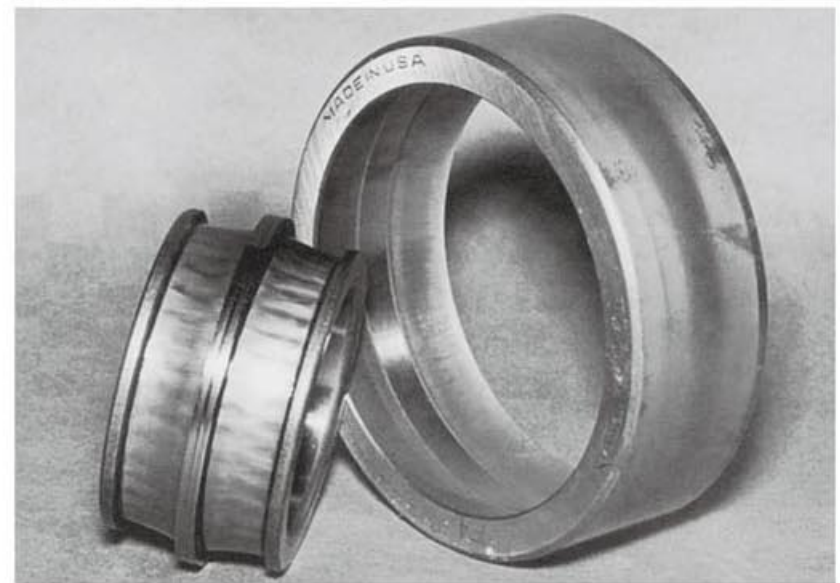
Figure 31 ABRASIVE WEAR — INNER AND OUTER RING
