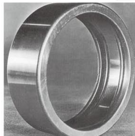
Figure 21 LUBRICATION FAILURE- RACEWAY
