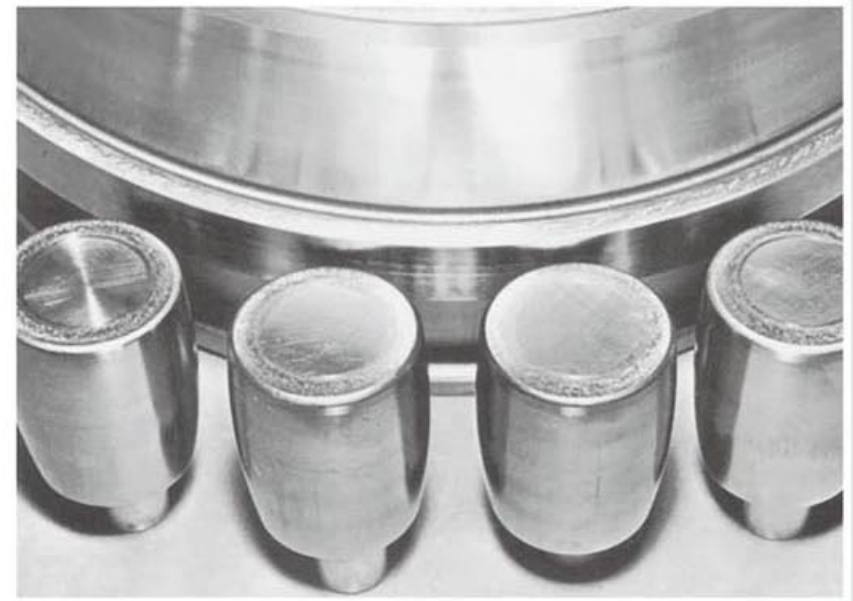
Figure 28 LUBRICATION FAILURE - THRUST CONTACT SURFACES
