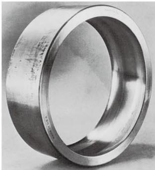
Figure 26 LUBRICATION FAILURE- OUTER RING
