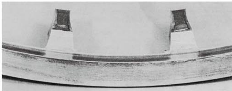
Figure 27 LUBRICATION FAILURE - RETAINER
