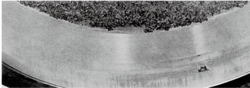
Figure 36 THRUST LOADING
