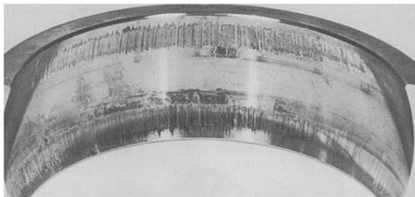
Figure 20 FALSH BRINELLING
