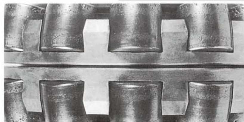
Figure 24 LUBRICATION FAILURE-ROLLERS
