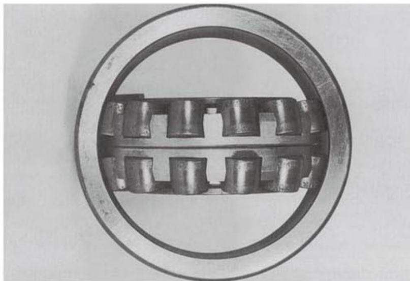
Figure 23 LUBRICATION FAILURE-ROLLERS
