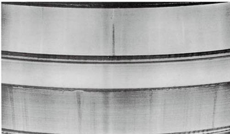
Figure 9 BRINELLED RACEWAY
