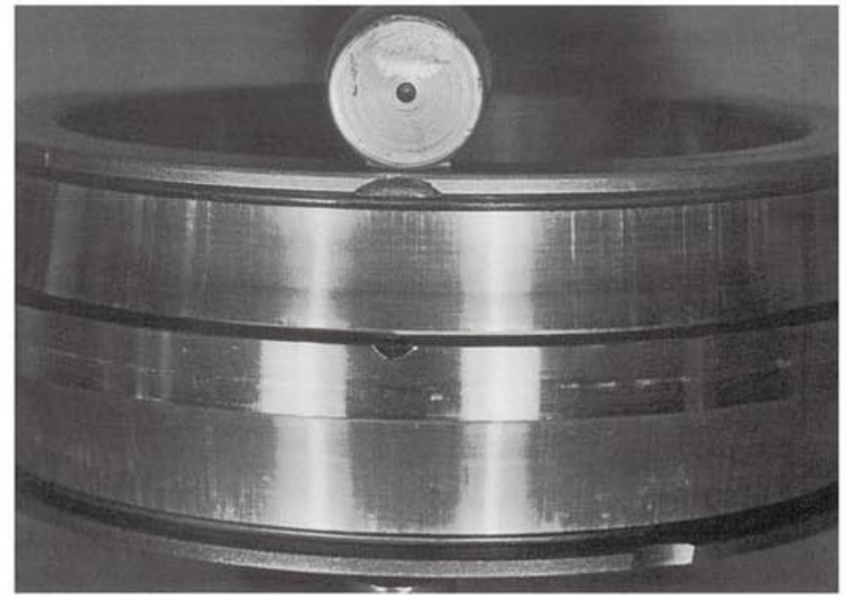
Figure 7 INSTALLATION DAMAGE
