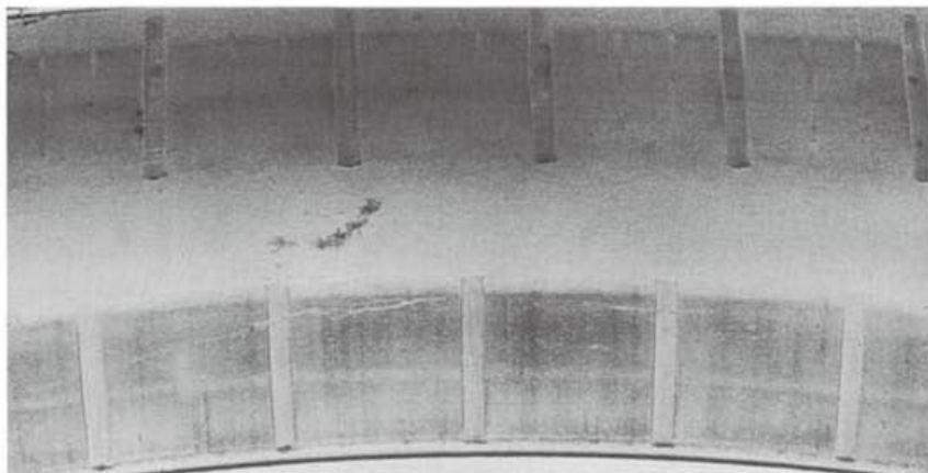
Figure 19 FALSH BRINELLING
